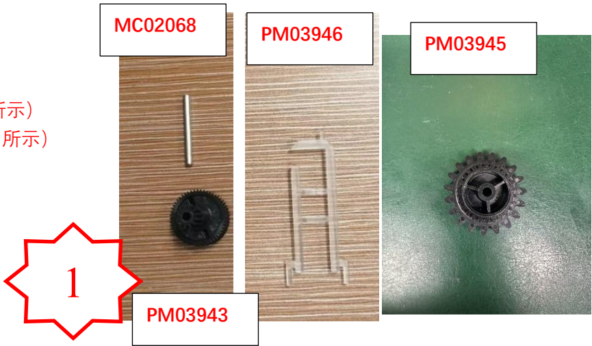
图一, 物料识别 PM03946, PM03943, MC02068, PM3945
